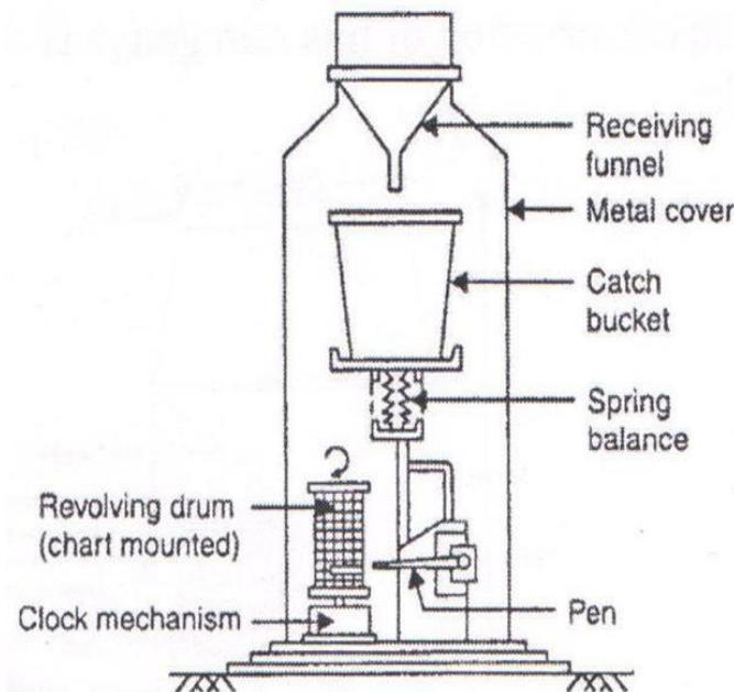
FIG: Weighing Bucket Rain gauge
