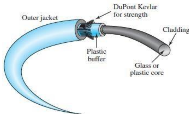
FIGURE 1.44: FIBER CONSTRUCTION
