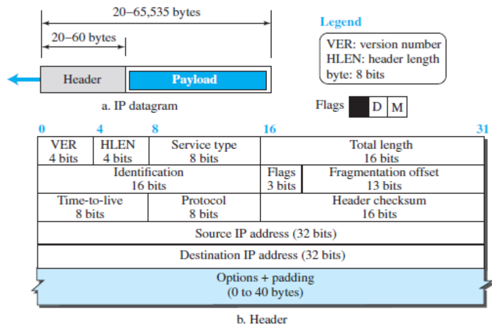
FIGURE 3.27: IP DATAGRAM
