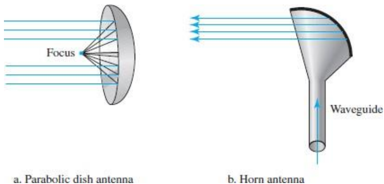
FIGURE 1.49: UNIDIRECTIONAL ANTENNAS
