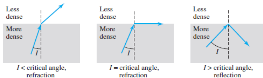
FIGURE 1.40: BENDING OF LIGHT RAY
