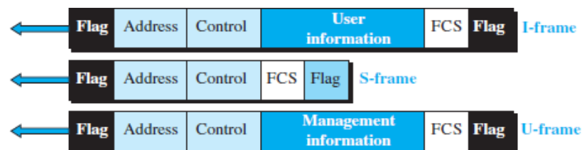
FIGURE 2.27: HDLC FRAMES
