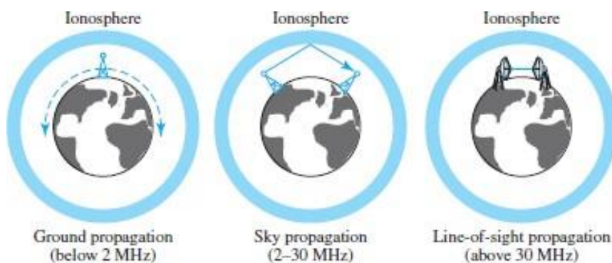
FIGURE 1.47: PROPAGATION METHODS
