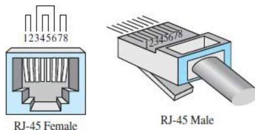
FIGURE 1.37: UTP CONNECTOR
