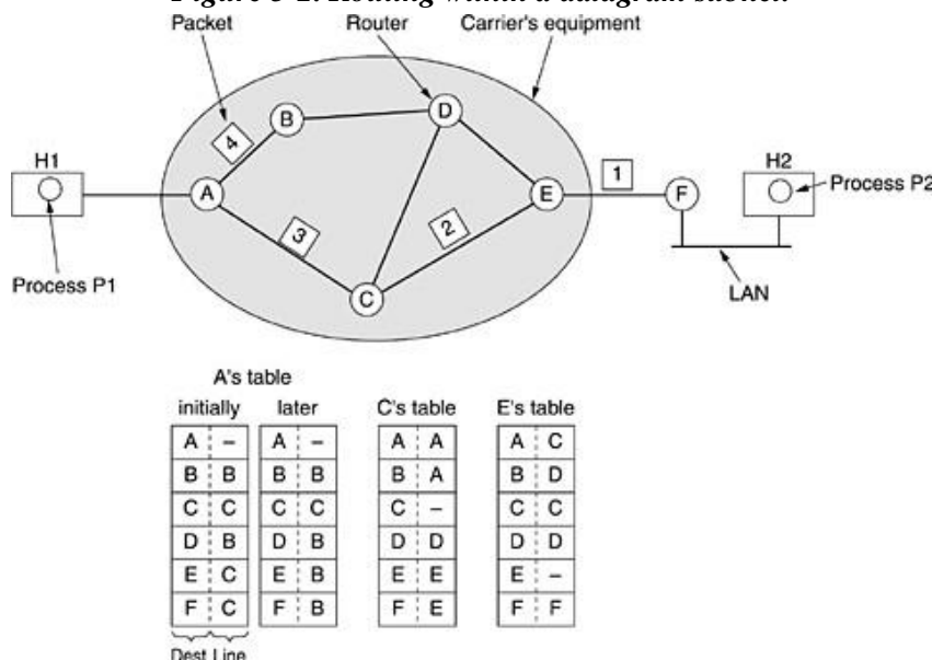
Figure 5-2. Routing within a datagram subnet.
