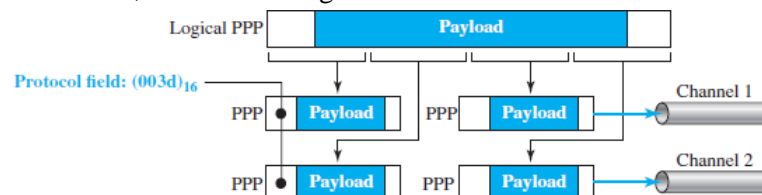
FIGURE: MULTILINK PPP
