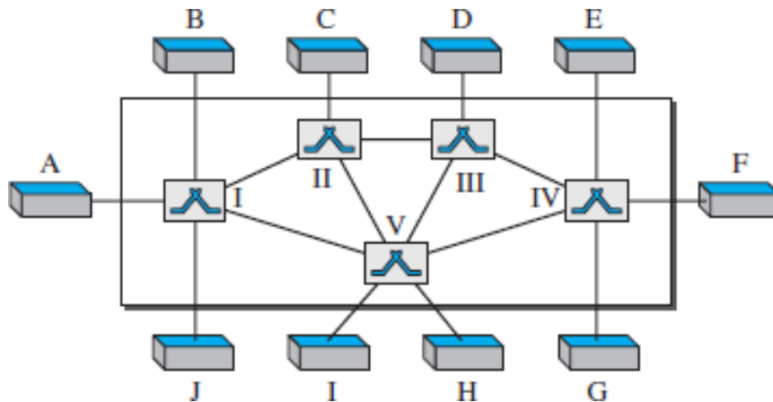
FIGURE 1.50: SWITCHED NETWORK
