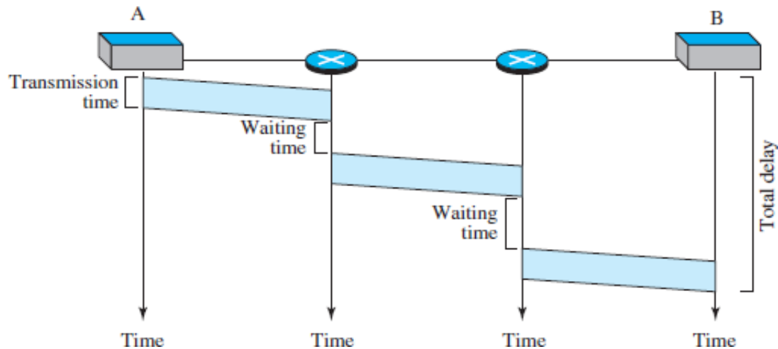
FIGURE 1.56: DELAY IN A DATAGRAM NETWORK
