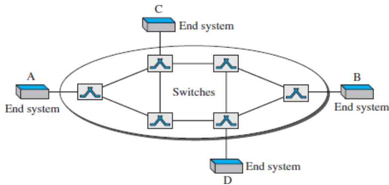
FIGURE 1.57: VIRTUAL-CIRCUIT NETWORK
