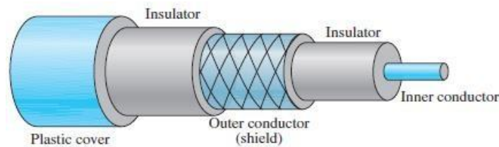
FIGURE 1.38: COAXIAL CABLE
