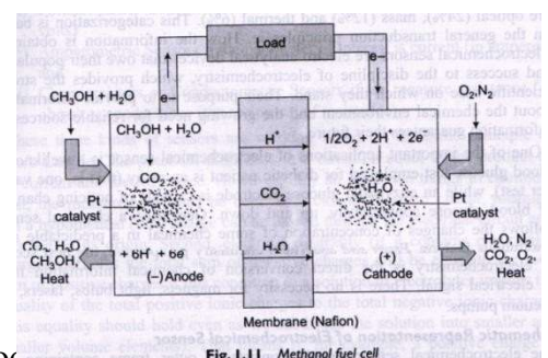
Fig. 1.11 Methanol fuel cell
