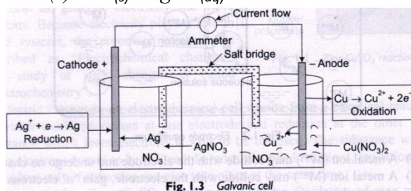
Fig. 1.3 Galvanic cell
