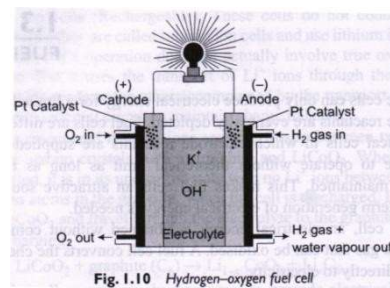
Fig. 1.10 Hydrogen-oxygen fuel cell
