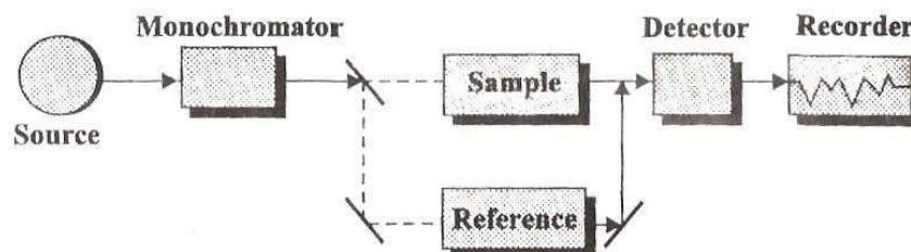
Block diagram of double beam IR spectrophotometer.
