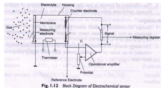
Fig. 1.12 Block Diagram of Electrochemical sensor
