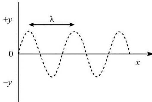
Figure 1. The wave motion in a string.
