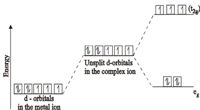
Fig1.18 Crystal field splitting of [\text{CoCl}_4]^{2-} complex
