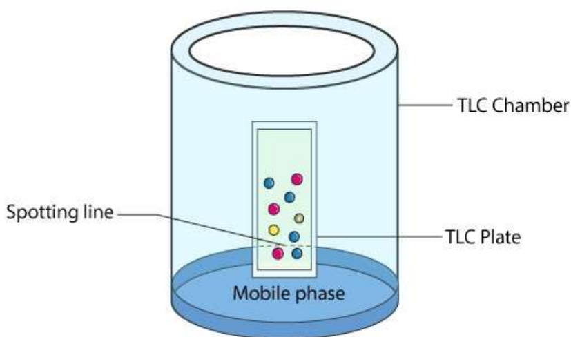
Diagram of Thin Layer Chromatography
