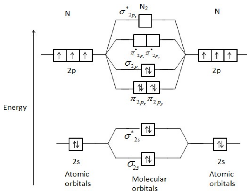
Fig: Molecular orbital diagram of N 2 molecule
